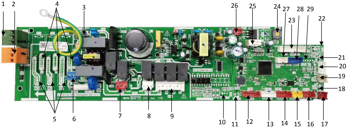
Figure 1.2: Four-way Cassette main PCB ports
