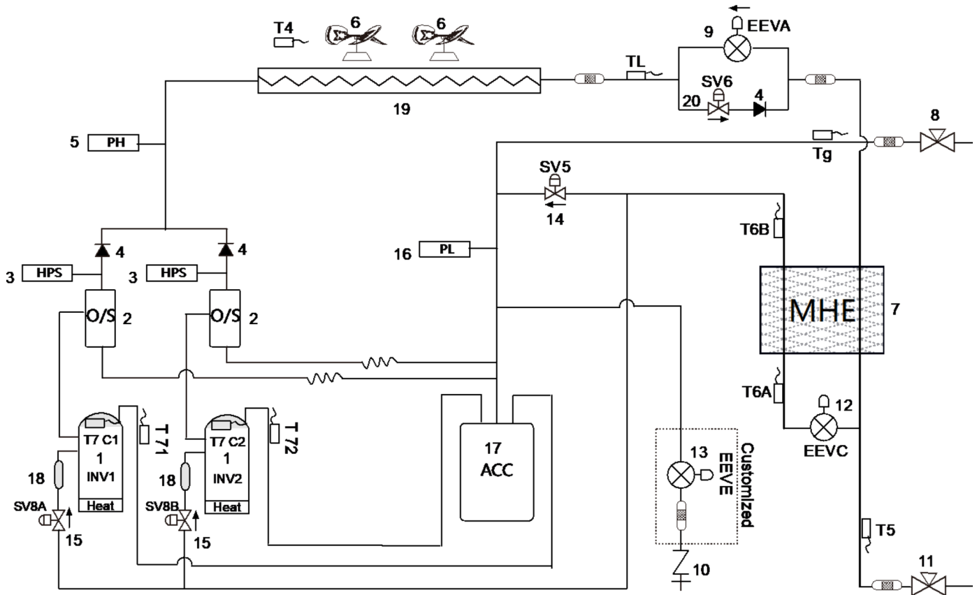
Figure 2-4.4: 26-30HP piping diagram
