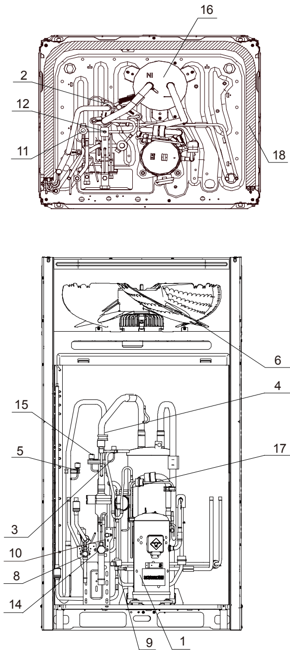
Figure 2-1.2: 14-20HP layout of functional components
