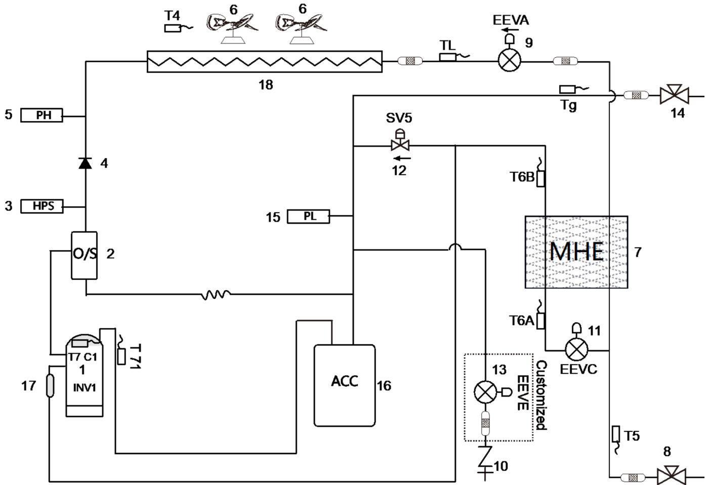
Figure 2-2.3: 22-24HP piping diagram
