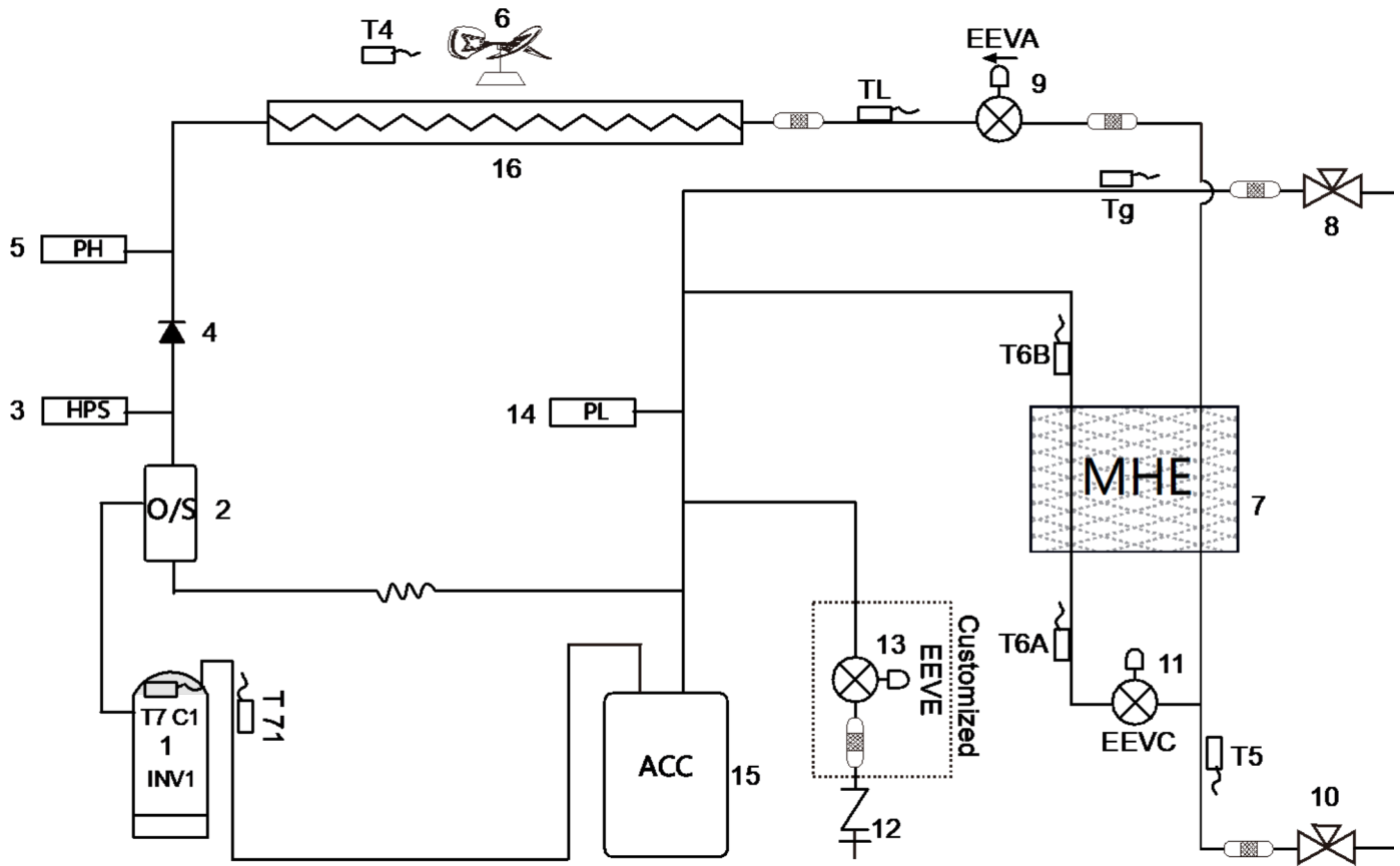
Figure 2-2.1: 8-12HP piping diagram
