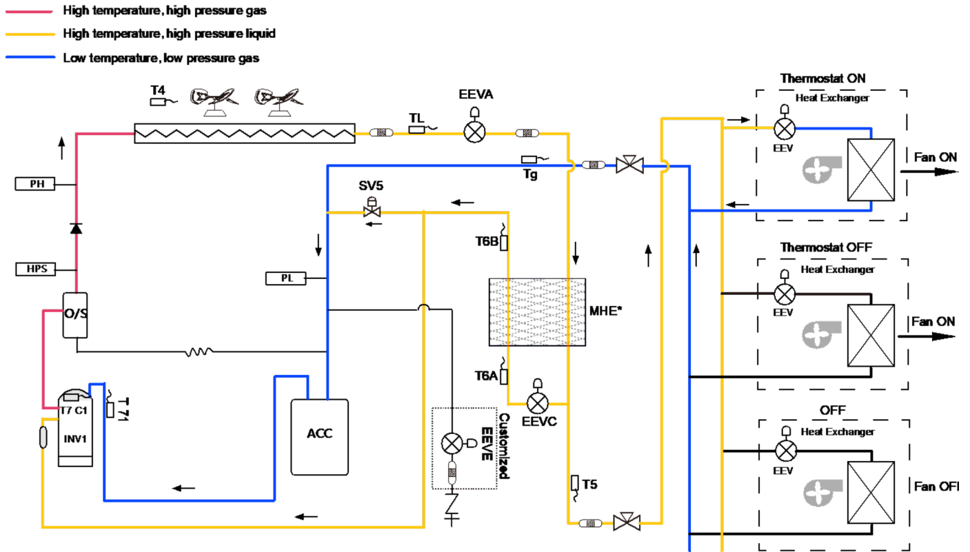
Figure 2-3.11: 22-24HP refrigerant flow during cooling operation
