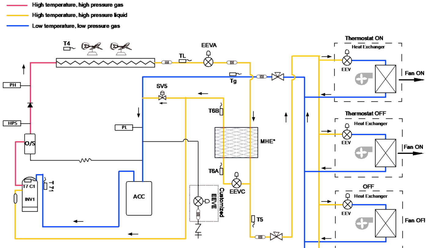
Figure 2-3.13: 22-24HP refrigerant flow during oil return operation in cooling mode
