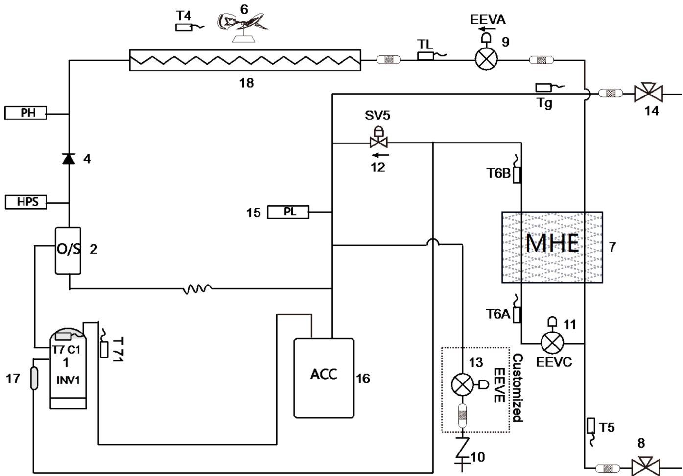
Figure 2-2.2: 14-20HP piping diagram
