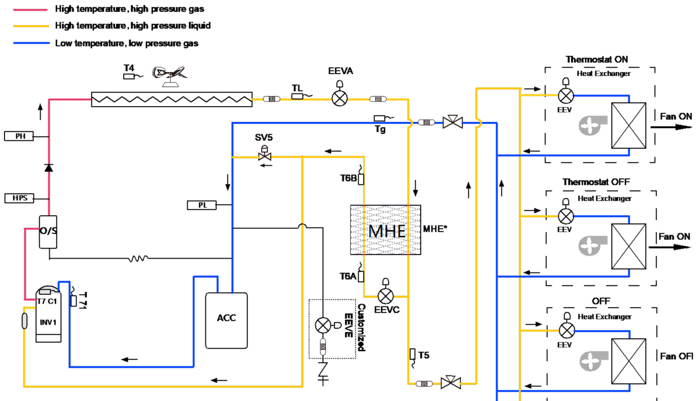
Figure 2-3.8: 14-20HP refrigerant flow during oil return operation in cooling mode
