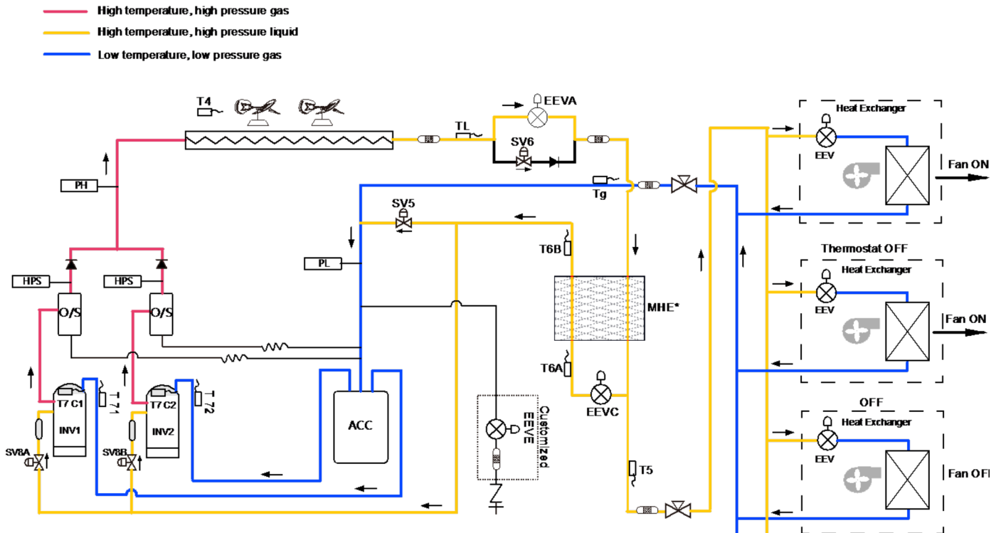
Figure 2-3.13: 26-30HP refrigerant flow during oil return operation in cooling mode
