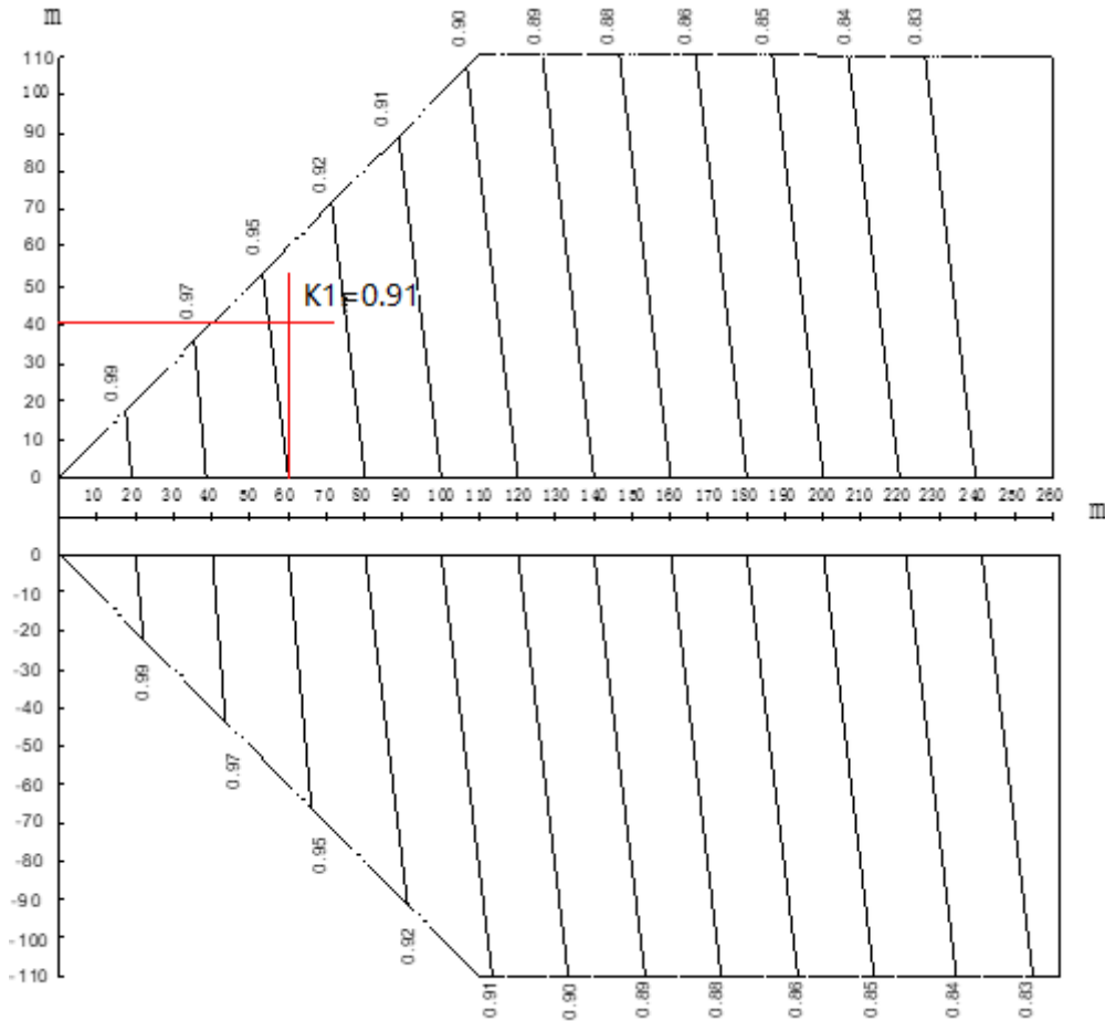
Figure 1-6.3: VC MAX rate of change in cooling capacity
