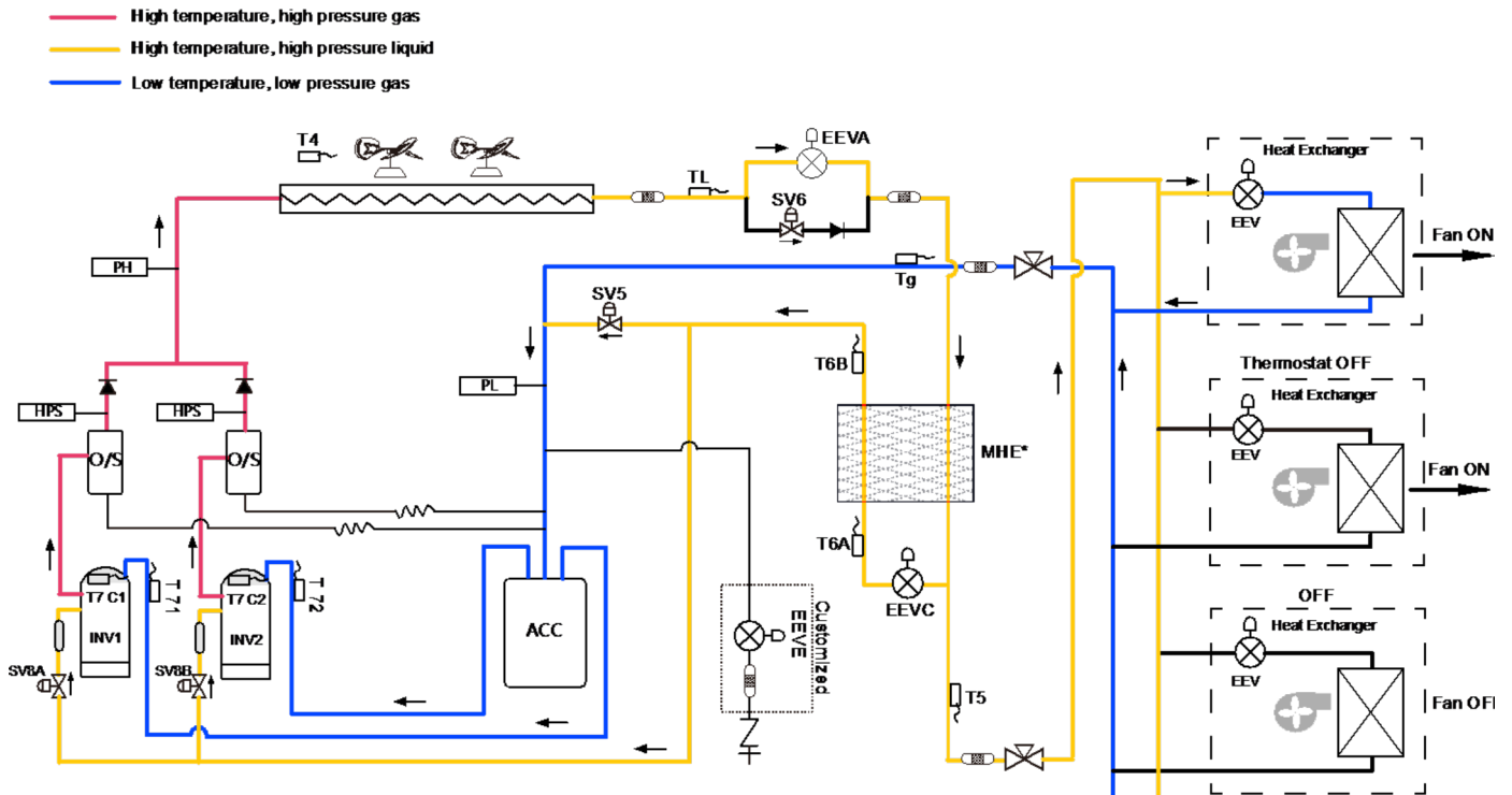
Figure 2-3.11: 26-30HP refrigerant flow during cooling operation
