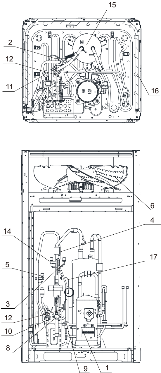
Figure 2-1.1: 8-12HP layout of functional components
