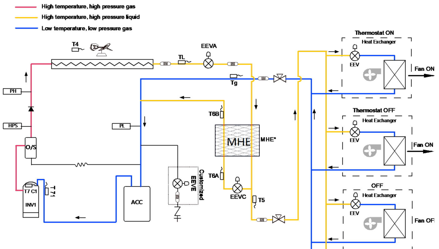
Figure 2-3.3: 8-12HP refrigerant flow during oil return operation in cooling mode
