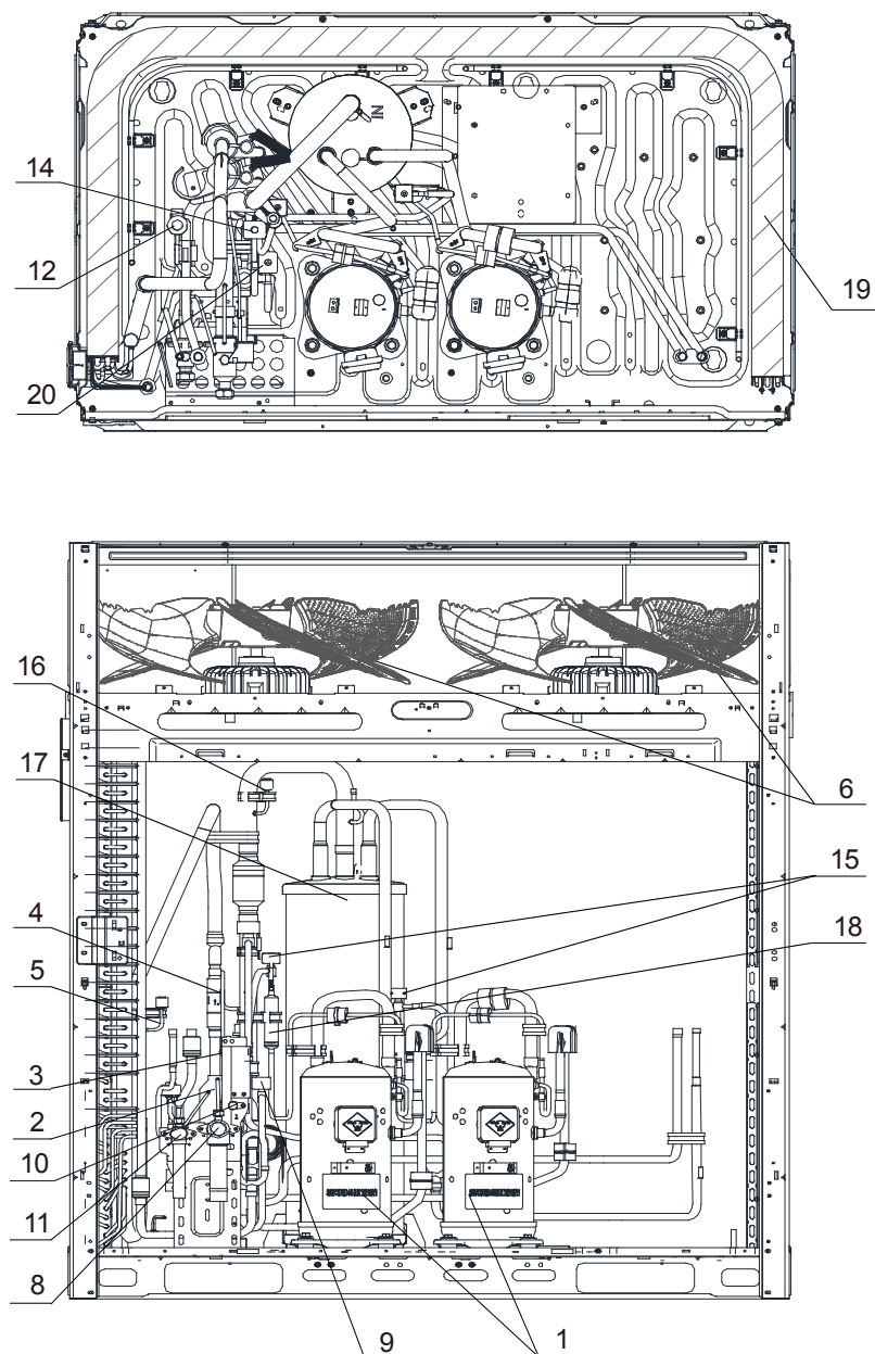
Figure 2-1.3: 26-30HP layout of functional components
