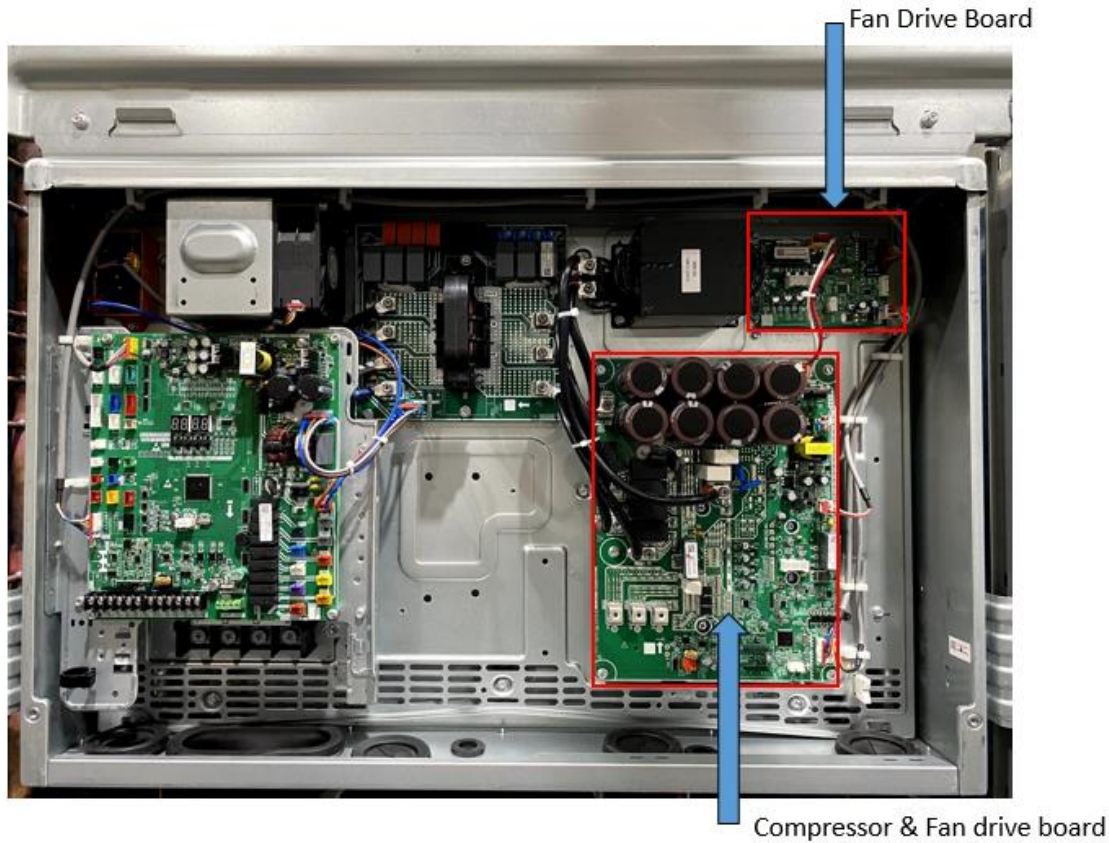
Figure 5-1.3: 22-24HP electric control box
