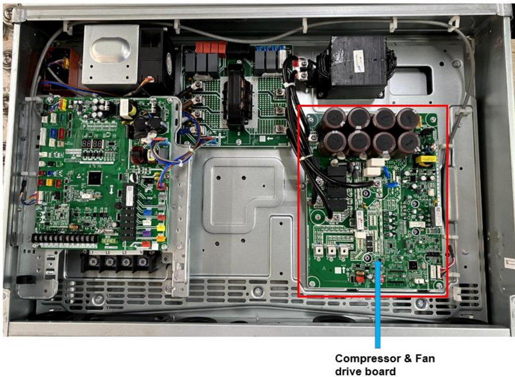
Figure 5-1.2: 20HP electric control box
