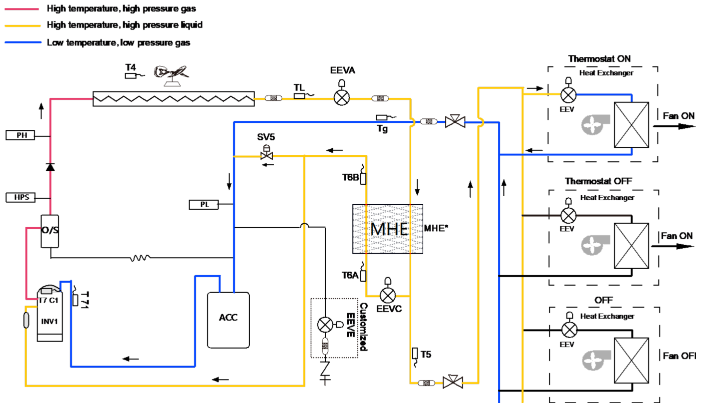
Figure 2-3.6: 14-20HP refrigerant flow during cooling operation
