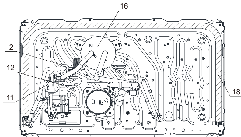
Figure 2-1.3: 22-24HP layout of functional components
