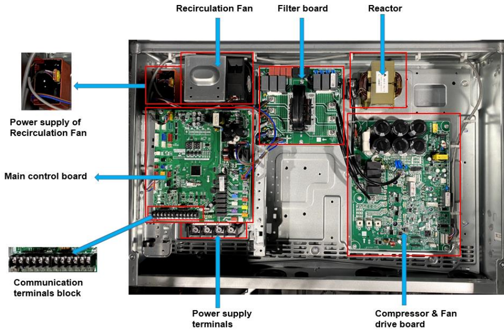
Figure 5-1.1: 8-18HP electric control box
