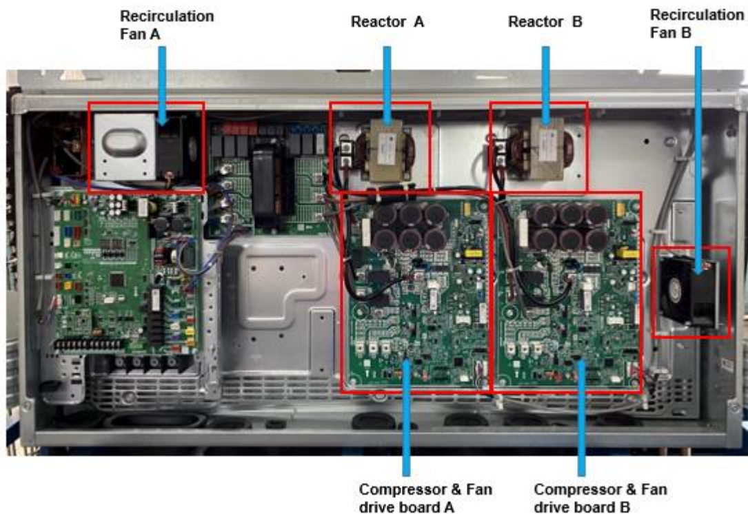
Figure 5-1.4: 26-30HP electric control box
