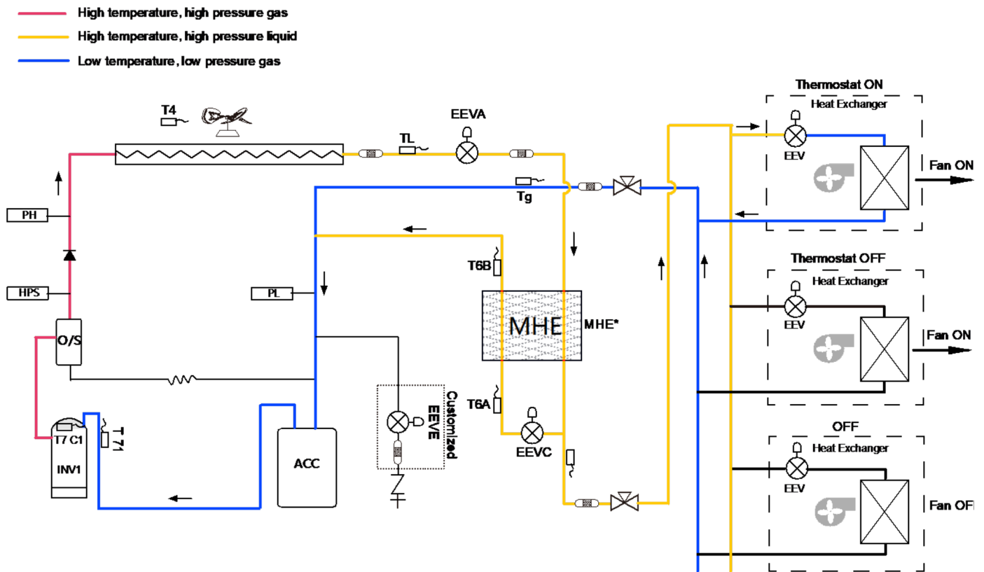
Figure 2-3.1: 8-12HP refrigerant flow during cooling operation
