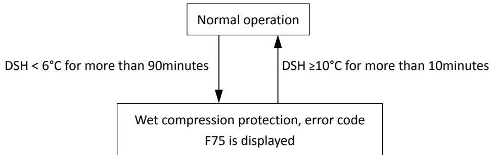
Figure 3-5.8: Wet compression protection control
