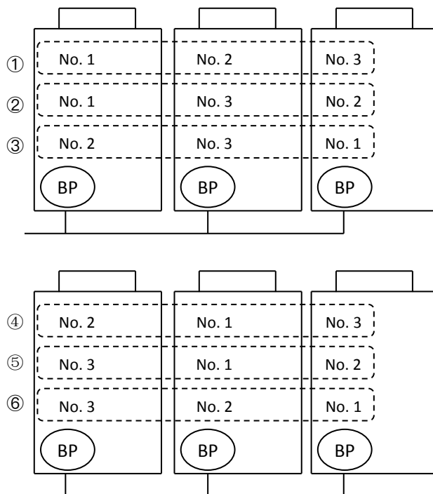
Figure 3-4.2: Compressor priority and rotation – three outdoor units
