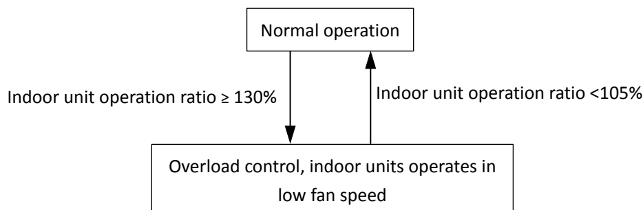
Figure 3-7.1: Overload control
