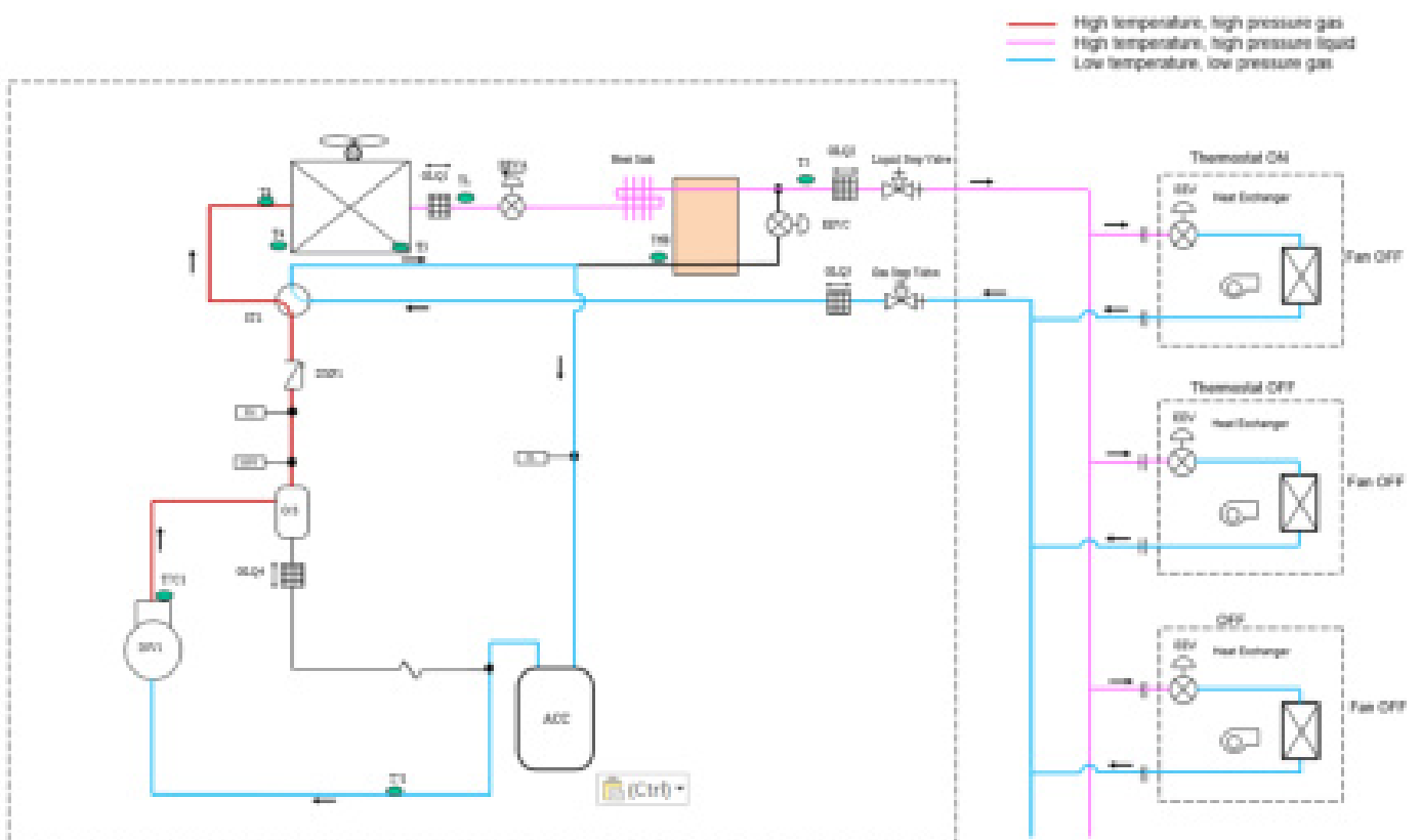
Figure 2-3.4: Refrigerant flow during oil return operation in heating mode and defrosting operation (4-way valve change direction)
