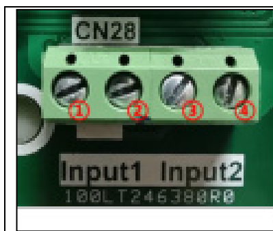
Figure A The dry contact is open (taking Input1 as an example)
