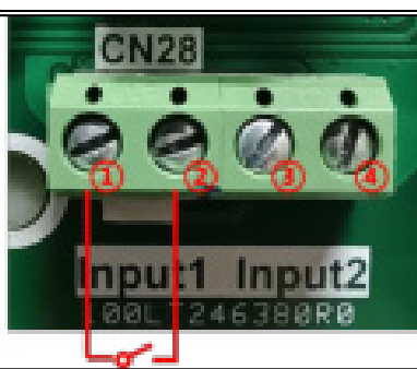
Figure A The dry contact is open (taking Input1 as an example)
