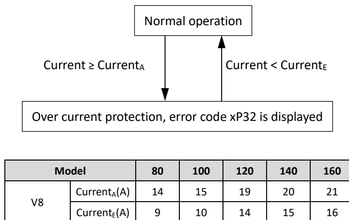
Figure 3-6.6: Over-current protection control
